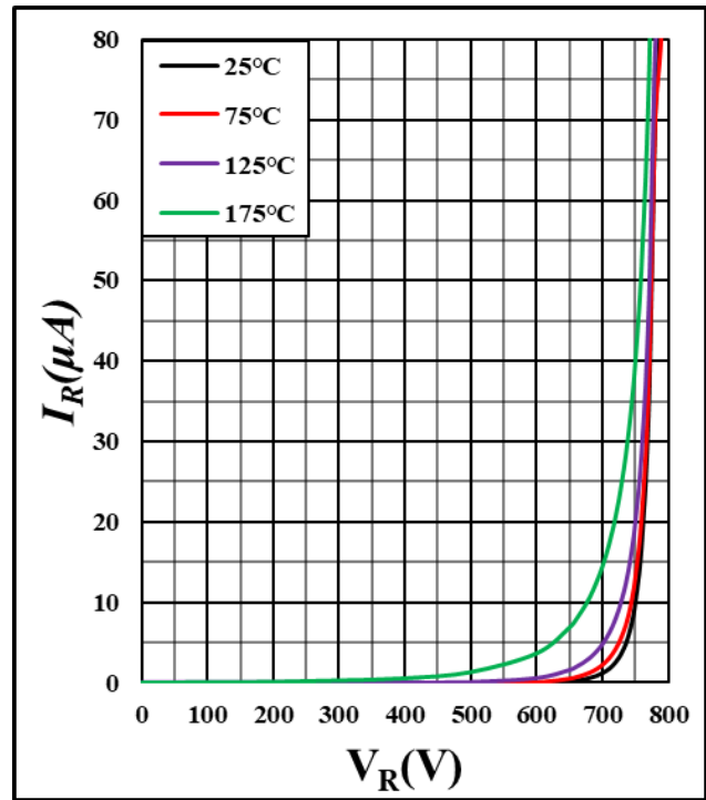
Figure 2. Reverse characteristics
