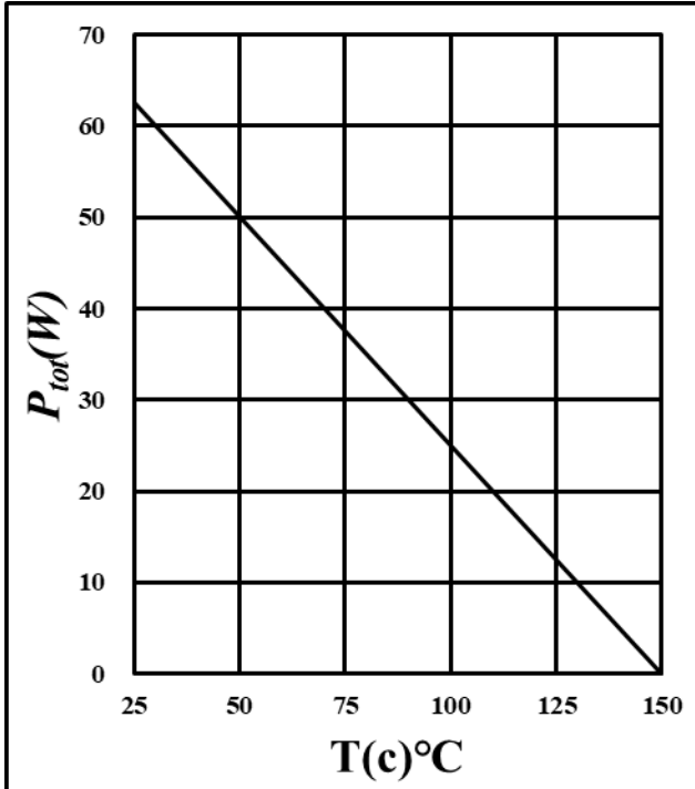
Figure 5. Power derating
