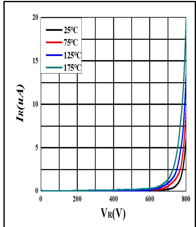
Figure 2. Reverse characteristics
