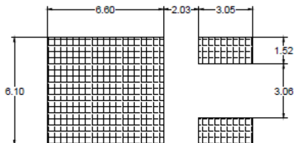
TO-252-2L
