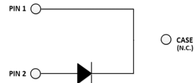
Package Type: TO-220F-2L
