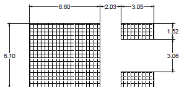
TO-252-2L
