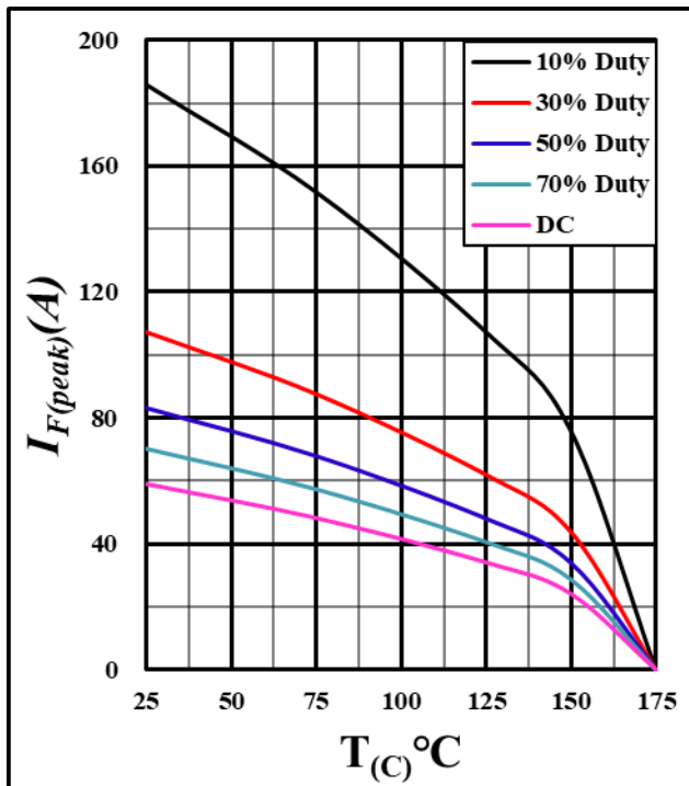
Figure 3. Current derating
