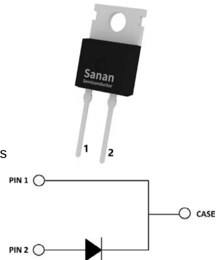
Package Type: TO-220-2L
