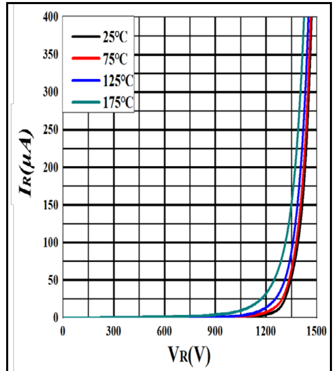
Figure 2. Reverse characteristics
