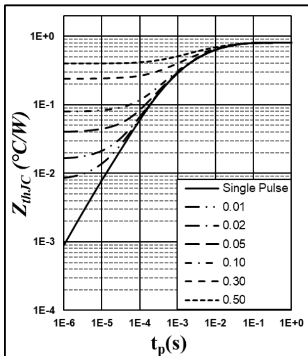
Figure 8. Transient Thermal Impedance (Junction - Case)
