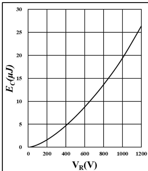
Figure 6. Capacitance stored energy
