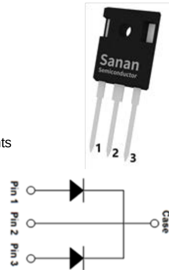
Package Type: TO-247-3L
