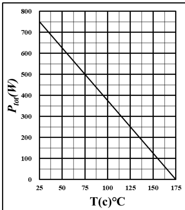
Figure 5. Power derating
