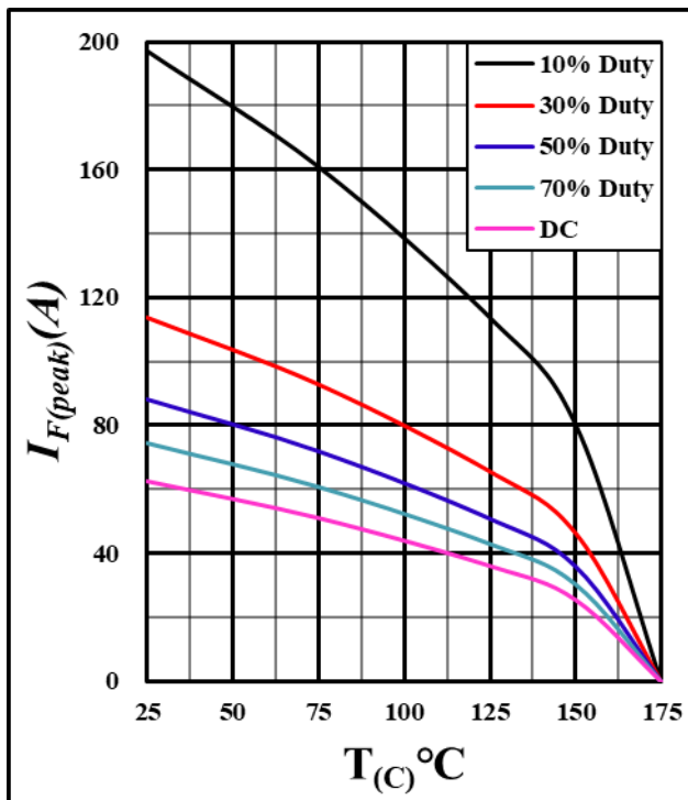
Figure 3. Current derating
