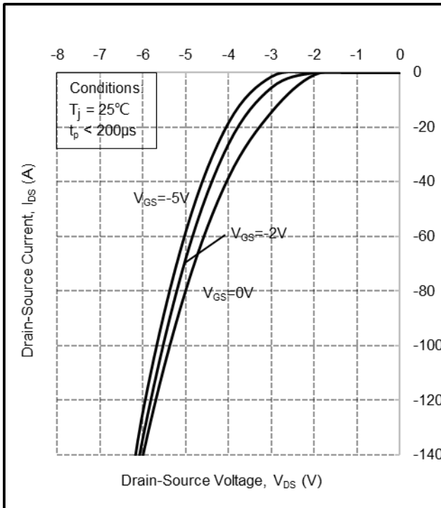
Figure 9. Body diode characteristic at T_j = 25^\circ\text{C}
