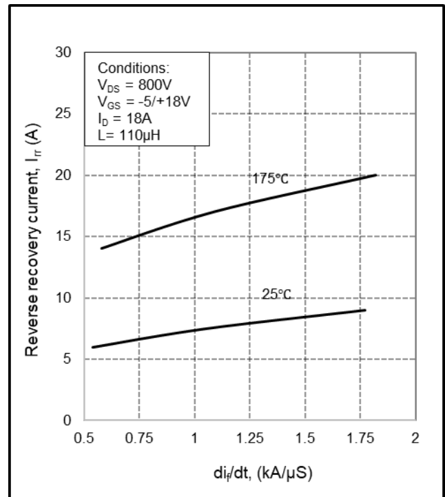
Figure 26. Reverse recovery current vs. di_T/dt
