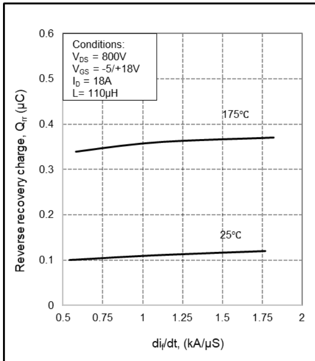
Figure 25. Reverse recovery charge vs. di_T/dt
