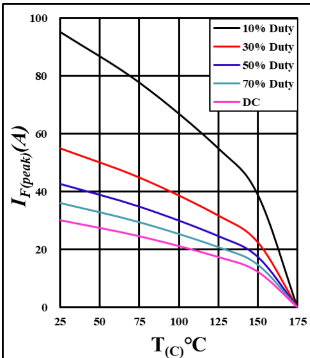
Figure 3. Current derating
